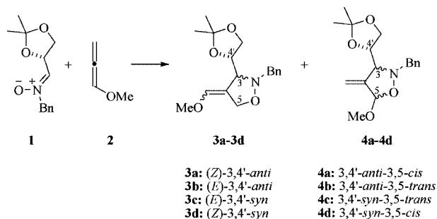
Scheme 3. 1,3-Dipolar cycloadditions of D-glyceraldehyde-derived nitronene 1 with methoxyallene ( 2 ).
