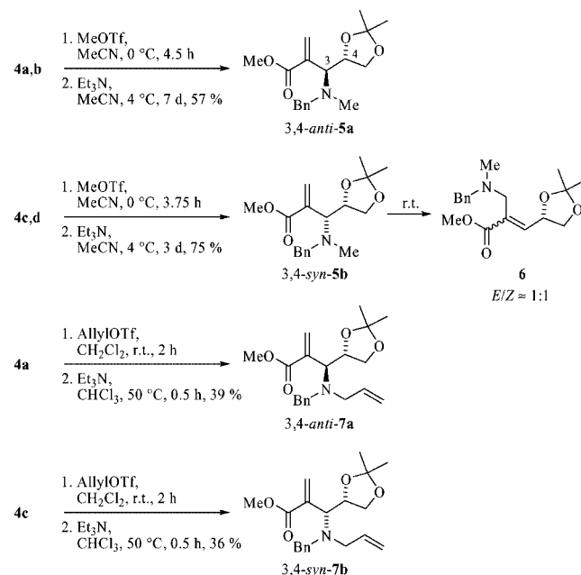
Scheme 5. Redox ring-opening of isoxazolidines 4a–4d by treatment with alkylating agents and base.
