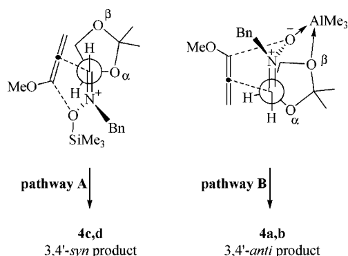
Scheme 4. Pathways of Lewis-acid-promoted cycloadditions of nitrone 1 with methoxyallene.
