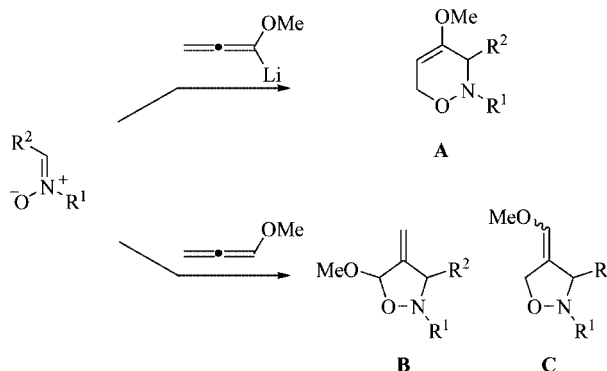
Scheme 1. Nucleophilic addition of lithiated methoxyallene to nitrones leading to 1,2-oxazines A and cycloaddition pathways providing isoxazolidines B or C .
