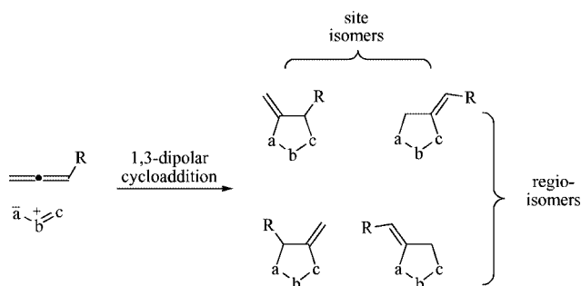
Scheme 2. Site- and regioselectivity in 1,3-dipolar cycloadditions of nitrones with monosubstituted allenes (stereoisomers are not shown).
